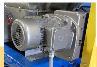
Oversized Extruder Gearbox with AC Drive and Inverter Duty Motor
